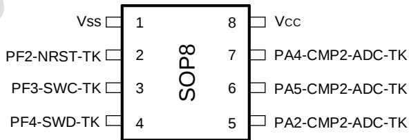
图 3-11 SOP8 Pinout1 PY32T020L1xS7-B (Top view)
